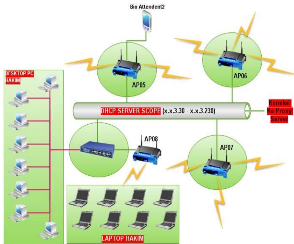
GAMBAR 3.22 BACKBONE WIFI NETWORK LANTAI 3 PTA BANDUNG
