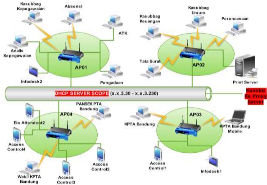
GAMBAR 3.21 BACKBONE WIFI NETWORK LANTAI 2 PTA BANDUNG
