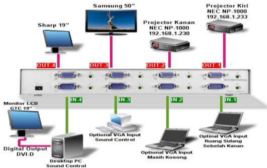
GAMBAR 3.25 JARINGAN CONFERENCE SYSTEM PTA BANDUNG
