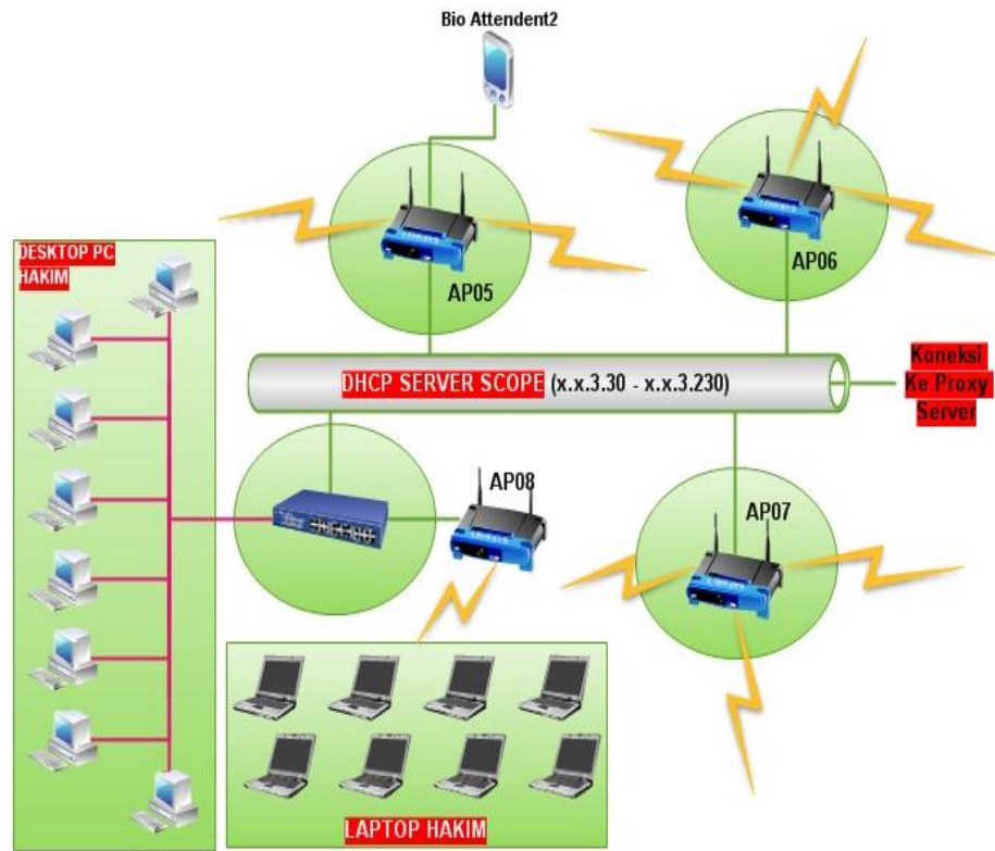
DIAGRAM 5.2 BACKBONE WIFI NETWORK LANTAI 3 PTA BANDUNG
