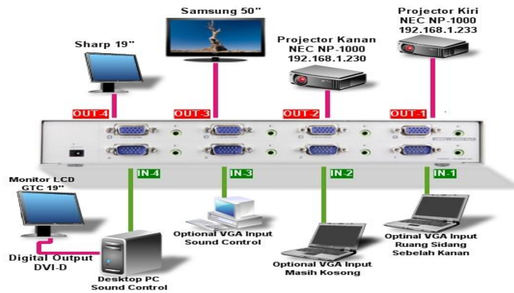
DIAGRAM 5.5 JARINGAN CONFERENCE SYSTEM PTA BANDUNG
