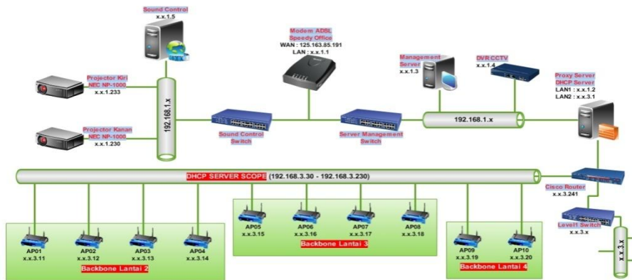
DIAGRAM 5.4 PETA KESELURUHAN BACKBONE WIFI NETWORK PTA BANDUNG
