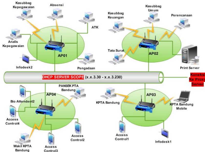
DIAGRAM 5.1 BACKBONE WIFI NETWORK LANTAI 2 PTA BANDUNG
